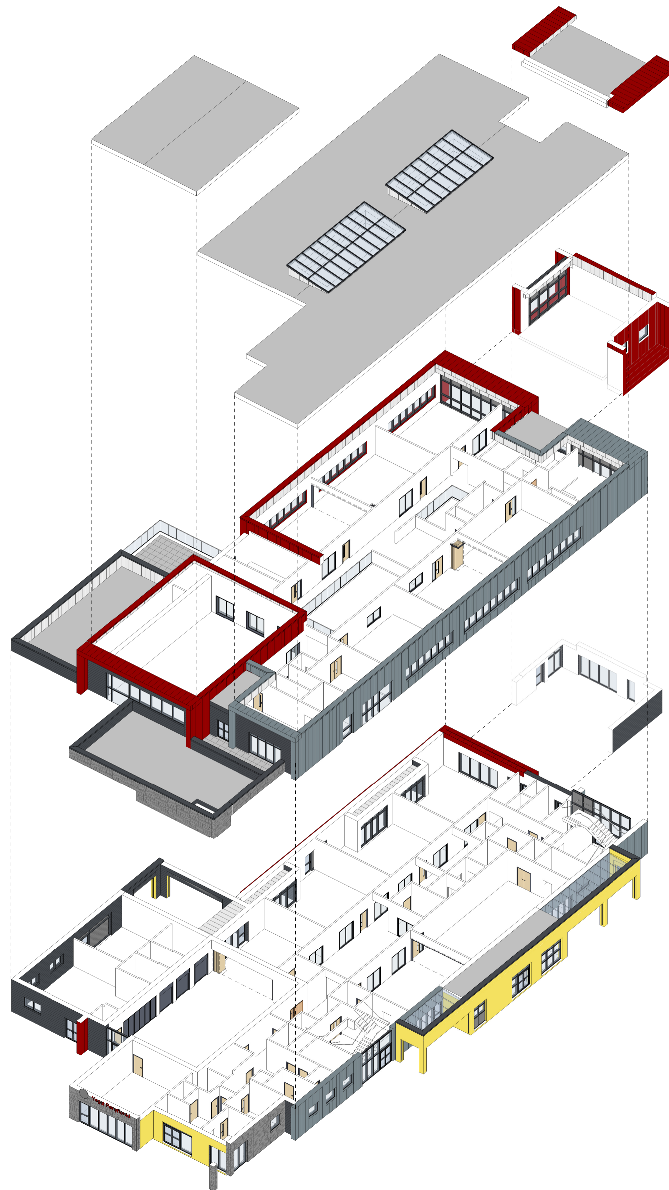
5 GA_Axonometric_ExplodedView_Phase02
